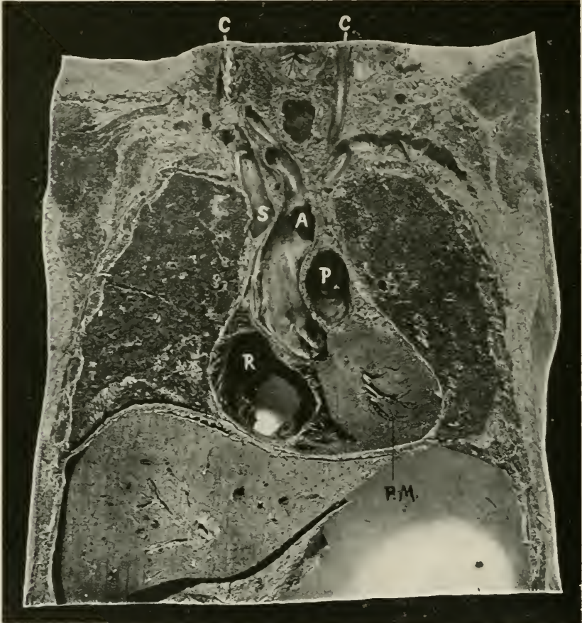
FIG. 180.—SECTION OF THE THORAX VIEWED FROM IN FRONT. Systolic (obstructive) aortic murmurs are transmitted in the direction of blood flow, upward into the carotid arteries. Systolic (regurgitant) mitral murmurs are transmitted in the opposite direction to the blood current, toward the left axilla, being conducted thence by the chordæ tendineæ and the papillary muscles. A = aorta; P = pulmonary artery; C = carotid arteries; P.M. = papillary muscle; R = right auricle; S = superior vena cava.
